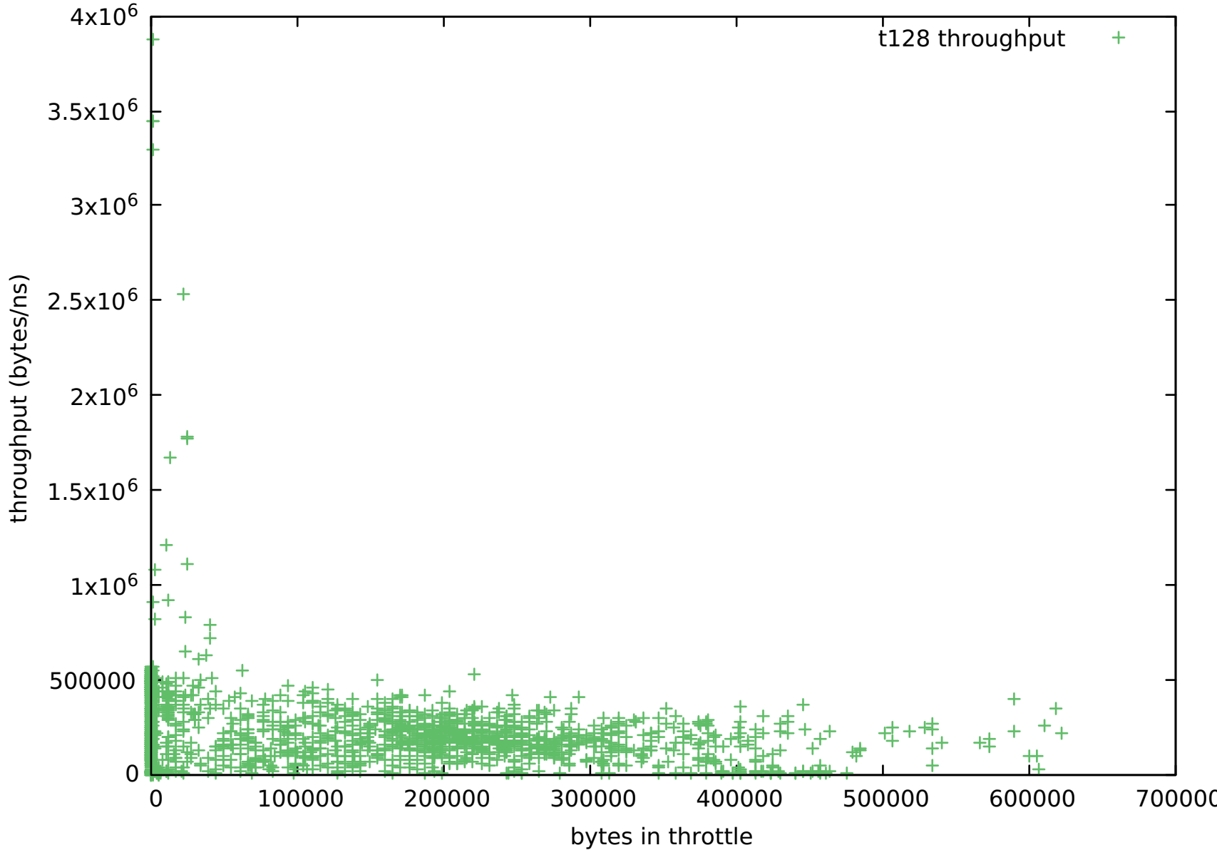
regbench-m t128 kv-sync throughput (bytes/ns)
